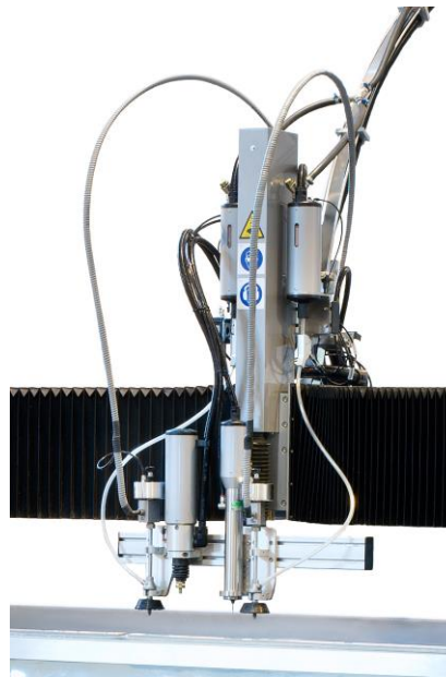
Single Z/Carriage Multi Head (Beam)
