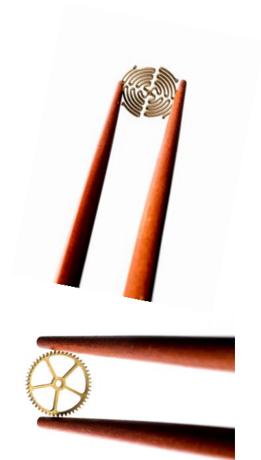
Fine Abrasive Waterjet Cutting (FAWJ)
